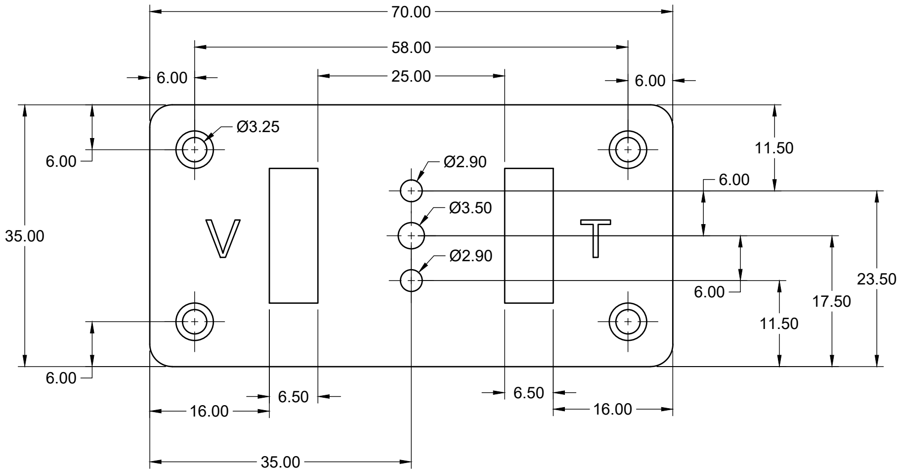
Vintage Preamp Top Plate Dimensions in mm.
